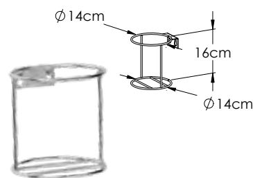
Support urinal inox mural
